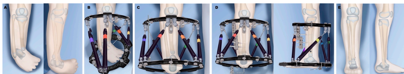
Figure 6. Treatment of Paley type 3A. (A) Distal tibia-fibula diastasis. The tibial plafond is absent and the end of the tibia is what normally would have been a medial malleolus; foot and fibula internally rotated around tibia. (B) Application of external fixator for gradual correction of foot and fibula position. (C) Foot centralized under end of tibia, ready for tibiotalar arthroplasty. (D) Distal tibia reshaping to talus and stabilization of distal tibia and fibula diastasis and osteotomy of tibia for diaphyseal straightening. (E) Final result after hardware removal with plantigrade foot and distal fibula screw epiphyseodesis.
